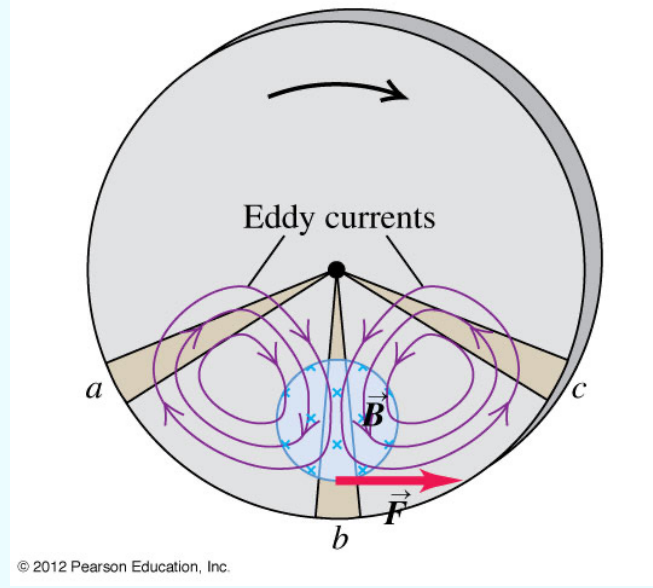
(b) Resulting eddy currents and braking force
