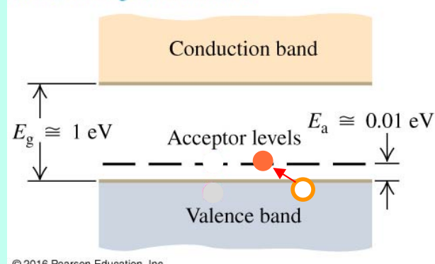
(b) Energy-band diagram for a p -type semiconductor at a low temperature. One acceptor level has accepted an electron from the valence band, leaving a hole behind.
