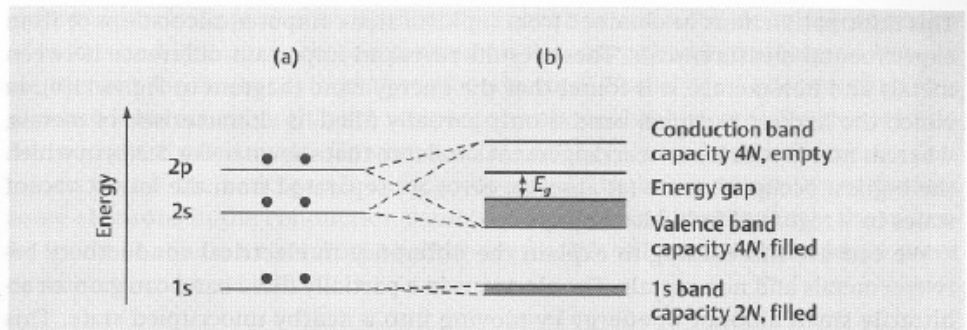
Figure 5.2 The occupation of (a) the energy levels in an isolated carbon atom, and (b) the energy bands in a diamond crystal. Notice that there is an energy range E_g separating the highest occupied states (in the valence band) from the lowest vacant states (in the conduction band). This is a characteristic feature of all insulators.
