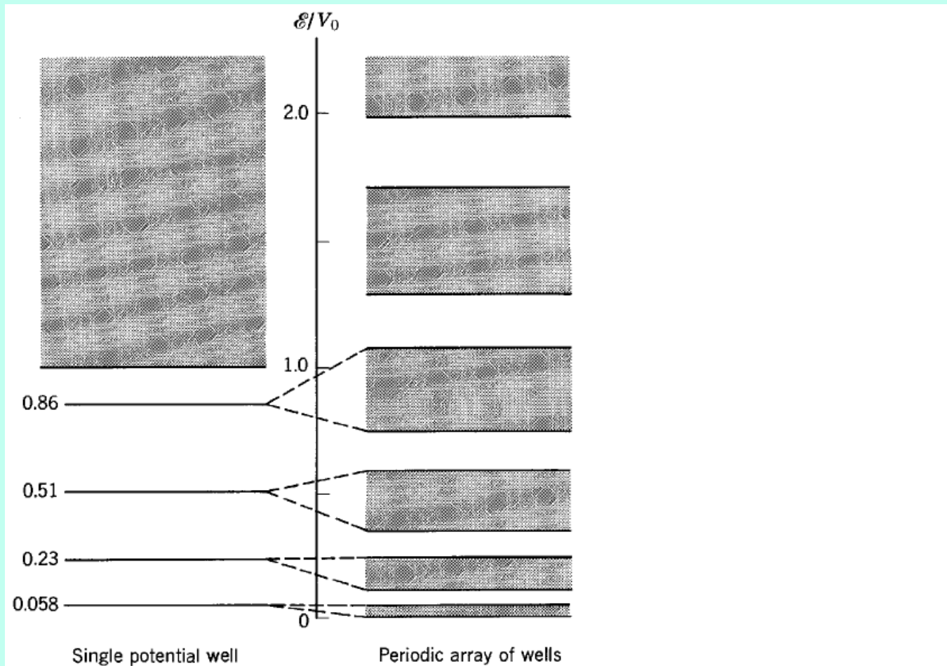
Figure 13-9 Left: Allowed energies for an electron in a single potential well. Right: Allowed energies in an array of periodically spaced wells and barriers. The levels shown are for a well strength given by 2mV_0l^2/\hbar^2 = (11)^2 , and a barrier thickness b = l/16 . Note the appearance of forbidden bands even for energies \epsilon greater than V_0 .
