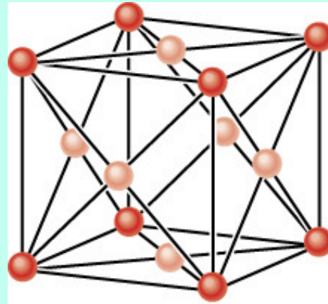
Copper fcc
