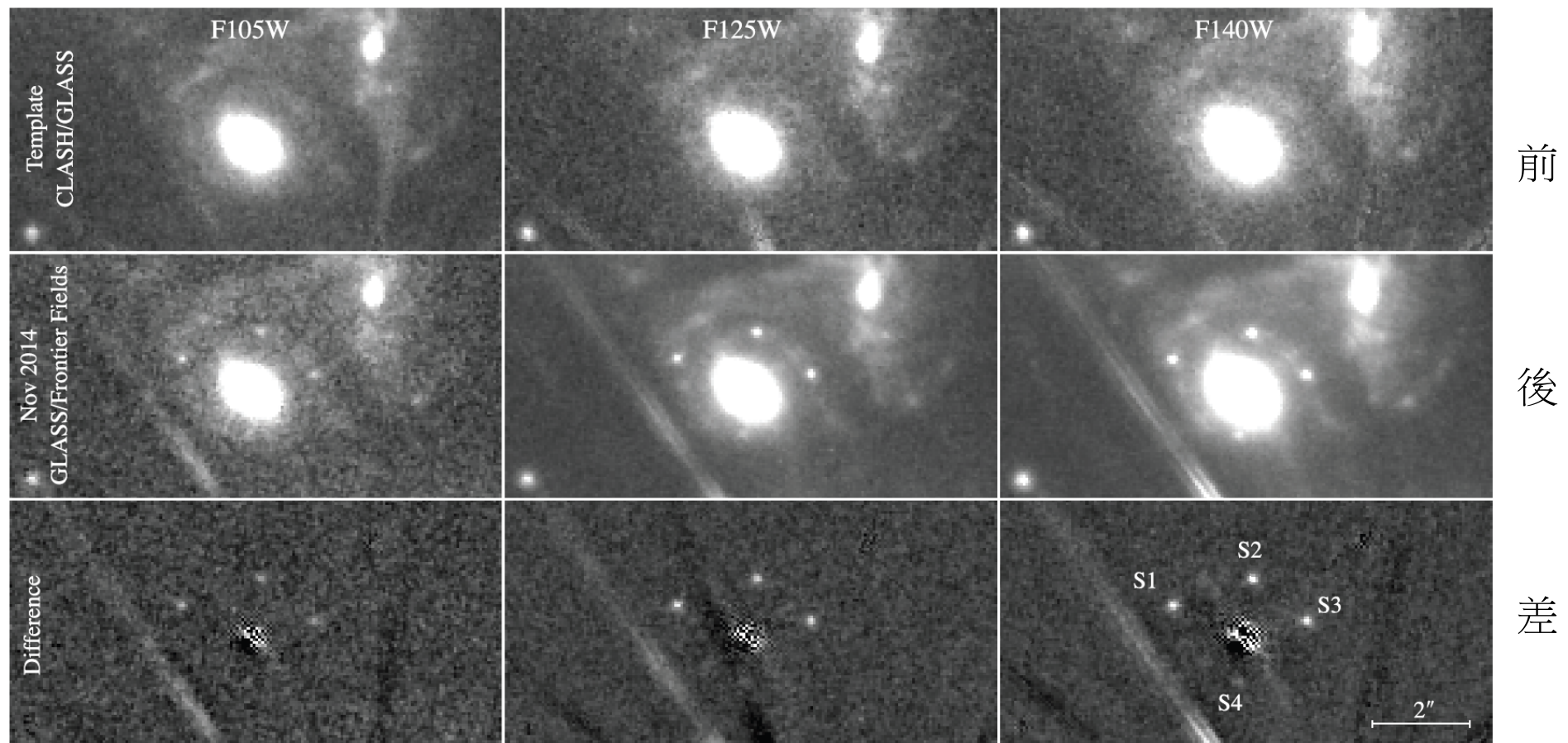
Fig. 1. HST WFC3-IR images showing the simultaneous appearance of four point sources around a cluster member galaxy. From left to right, the columns show imaging in the F105W filter (Y band), F125W (J), and F140W (JH). From top to bottom, the rows show archival imaging from the Cluster Lensing And Supernova survey with Hubble (CLASH, GO-12068; PI M.P.) program, discovery epoch images from GLASS and the Hubble Frontier Fields programs, and the difference images. The template images in the top row comprise all available archival WFC3-IR imaging in these filters, collected from
