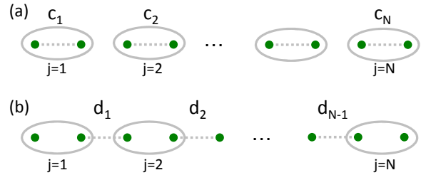
FIG. 2 A Kitaev chain with N sites and open ends. (a) A fermion operator c_j is composed of two MF operators. (b) Using a pair of MFs from different physical fermions to build a fermion operator d_j .
